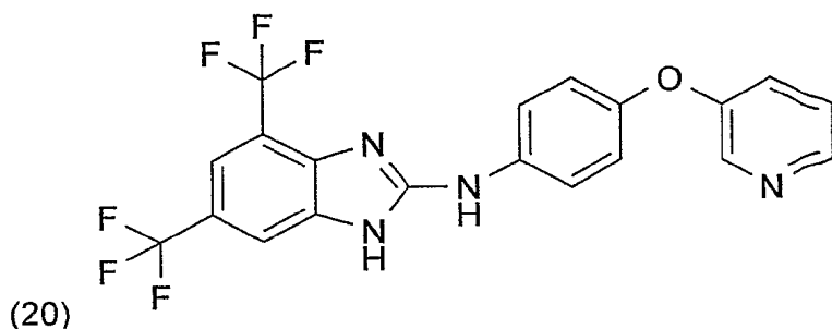
(20) (4,6-Bis-trifluoromethyl-1H-benzimidazol-2-yl)-[4-(pyridin-3-yloxy)-phenyl]-amin
